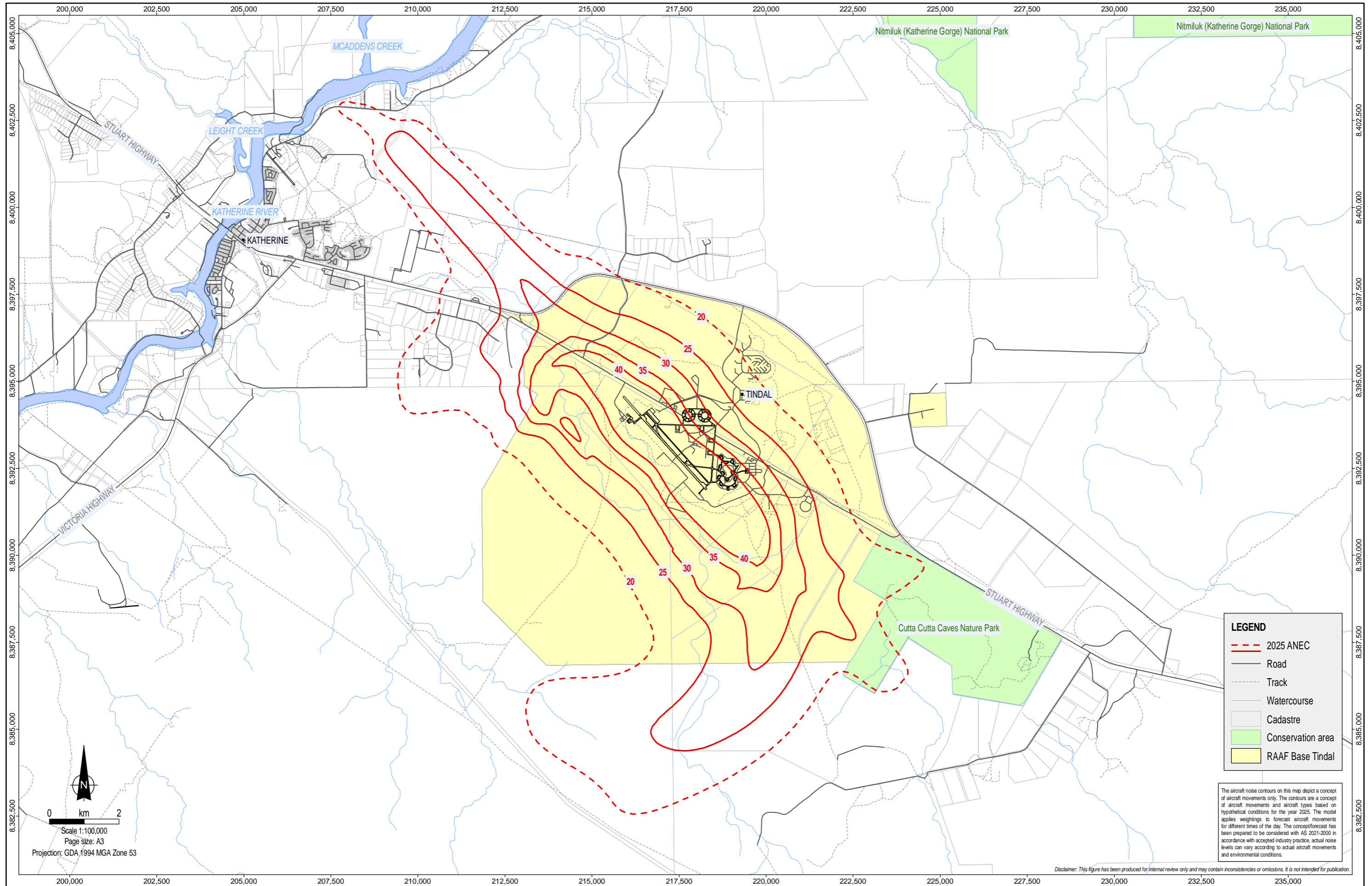
Figure 4: RAAF Base Tindal Noise Contours 2025 ANEC
